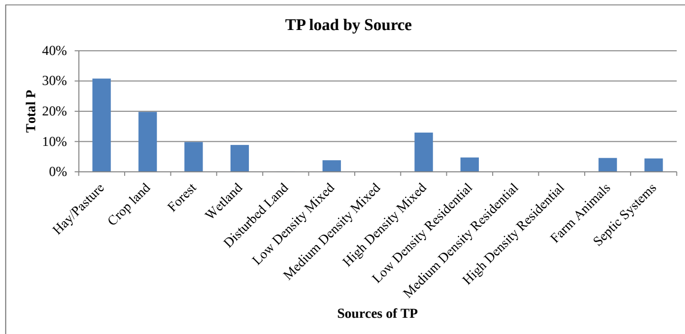
Figure 7: Total Phosphorus Loads by Source in the West Brook Watershed
