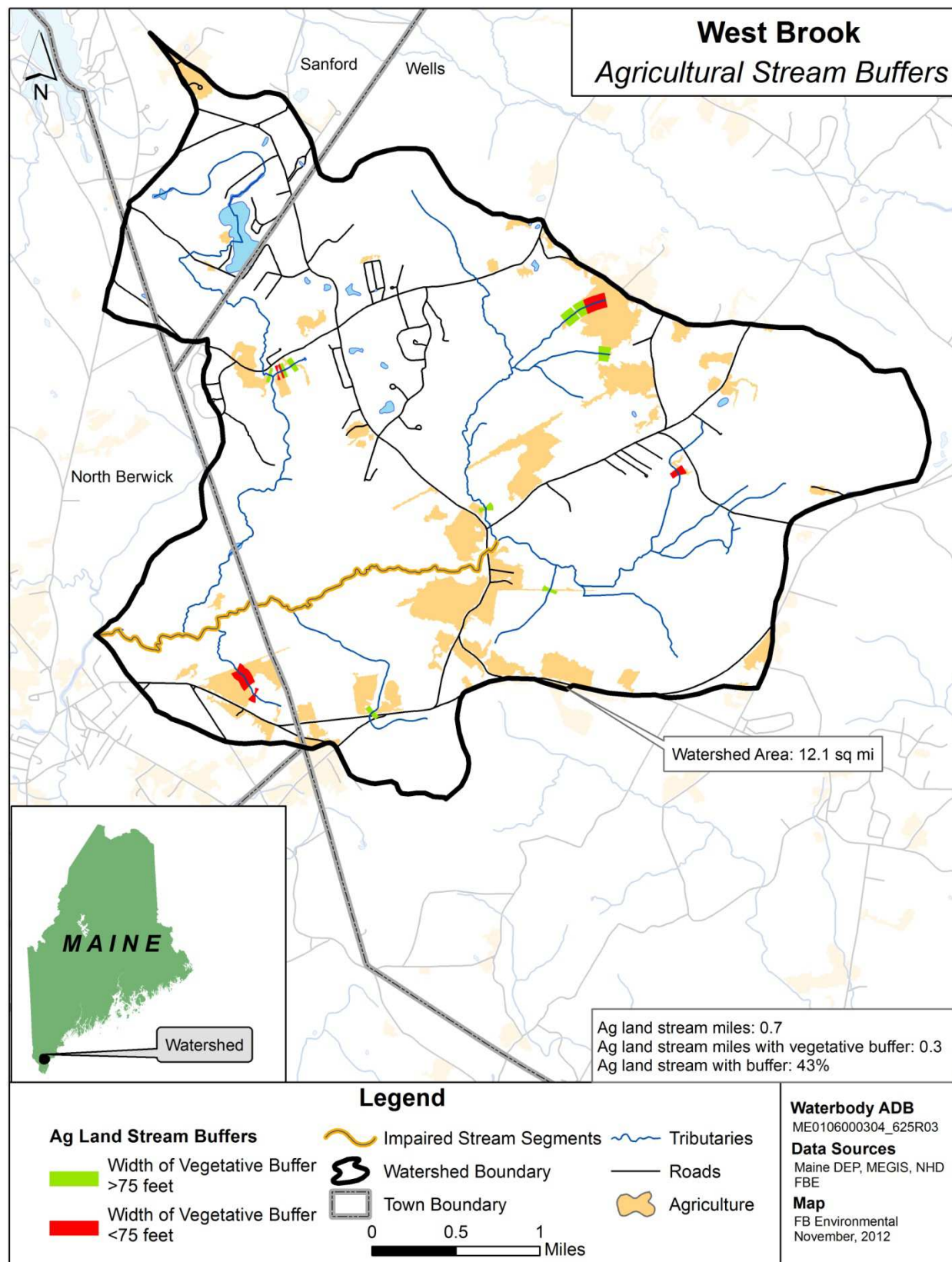
Figure 4: Buffered Agricultural Stream Miles in the West Brook Watershed
