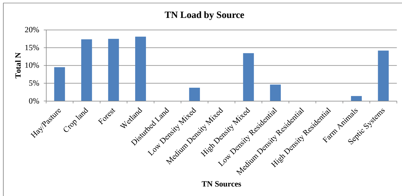
Figure 6: Total Nitrogen Loads by Source in the West Brook Watershed
