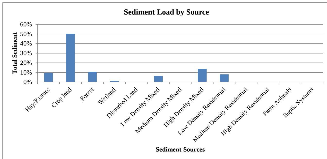
Figure 5: Total Sediment Loads by Source in the West Brook Watershed
