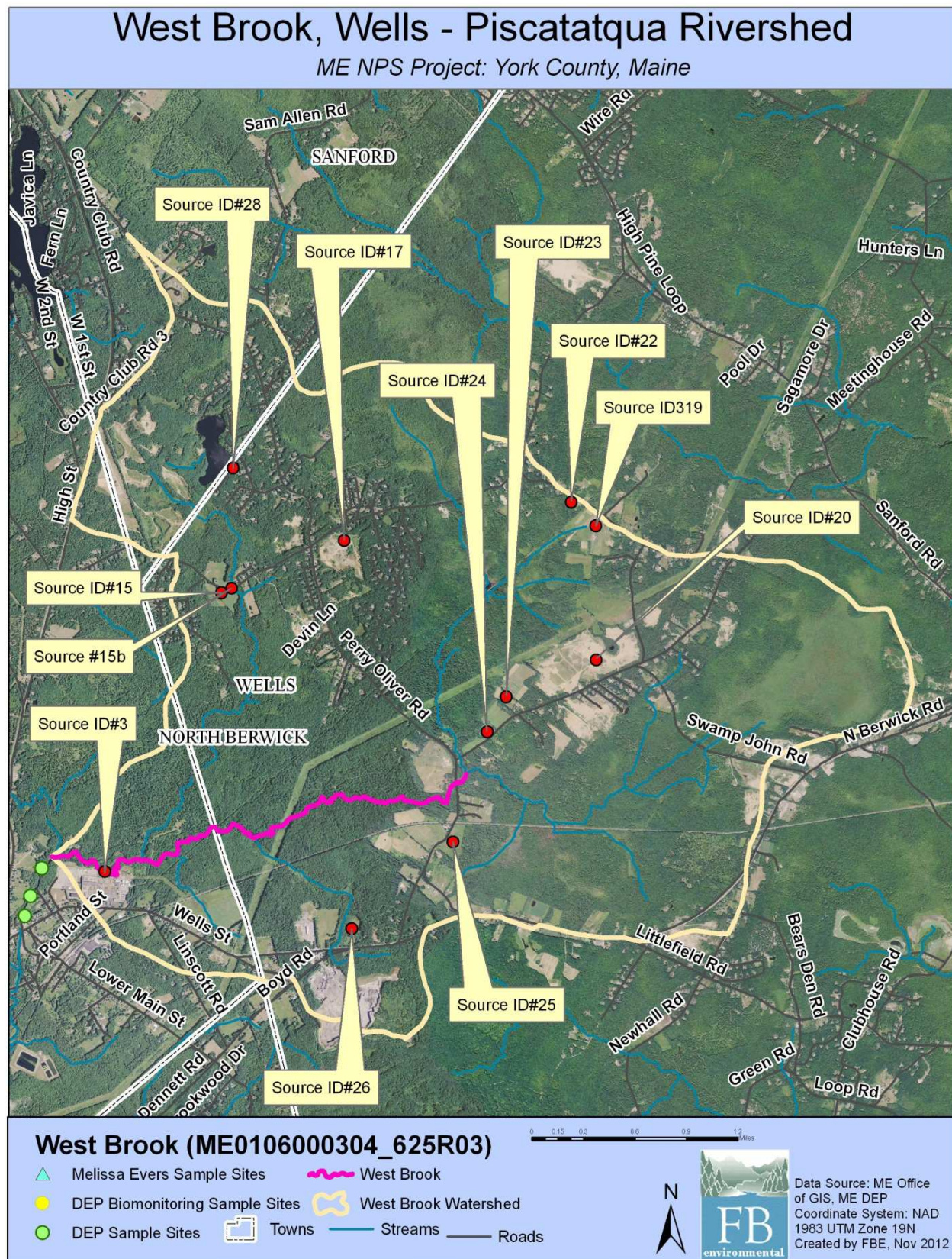
Figure 3: Aerial Photo of Source ID Locations in the West Brook Watershed
