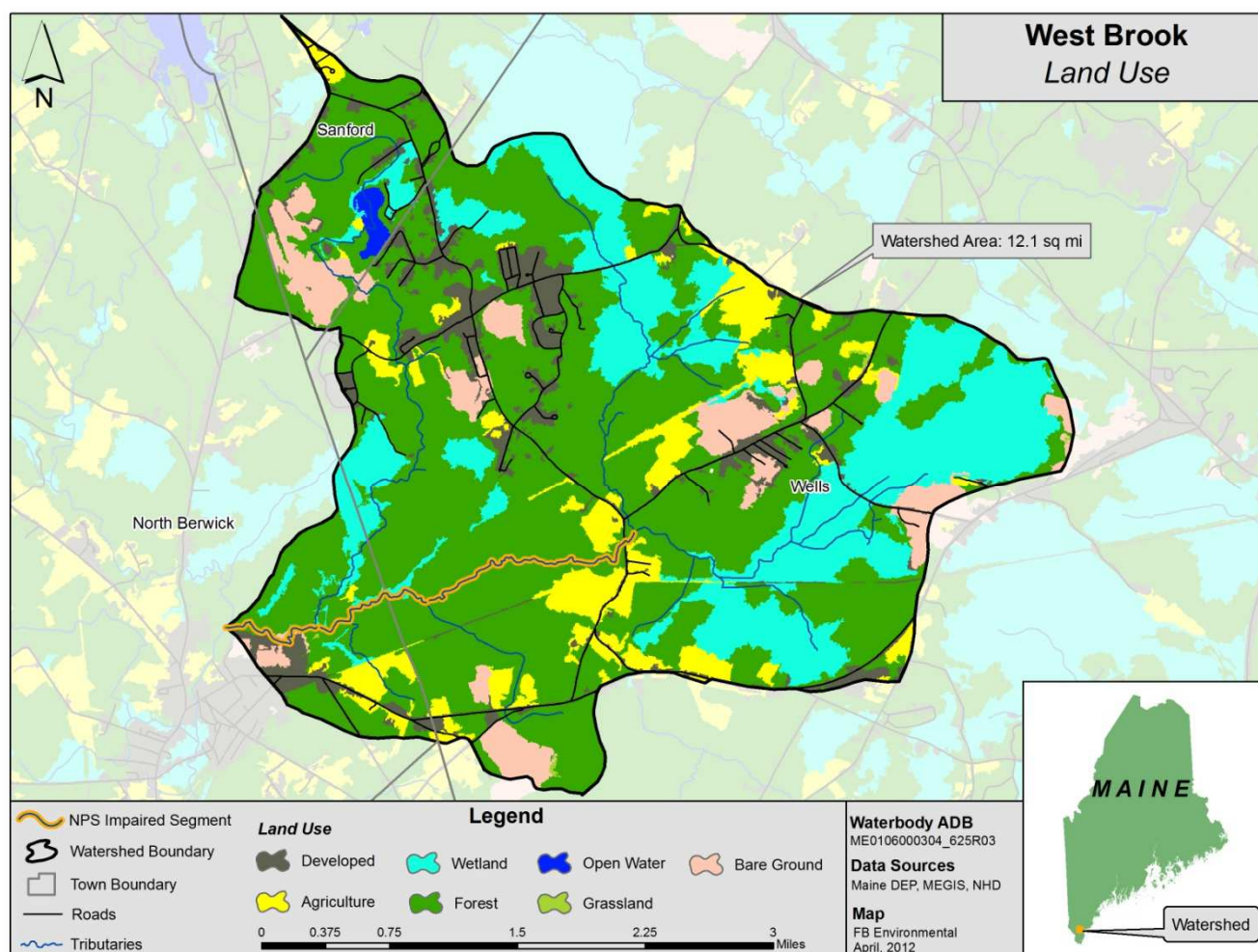
Figure 1: Land Use in the West Brook Watershed
