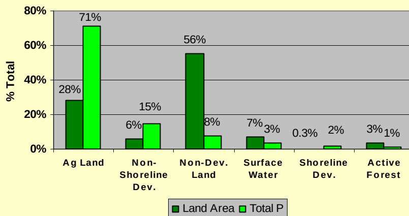
Figure 3: Land Use Areas and Phosphorus Loadings Lovejoy Pond Direct Watershed
