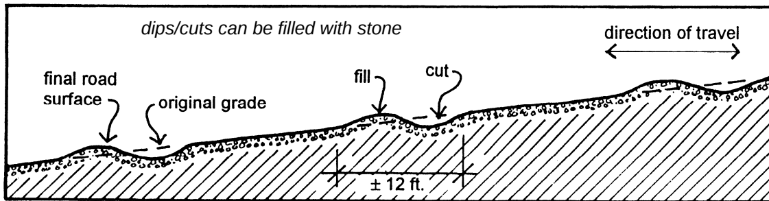
Figure 38. Water Bars
